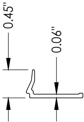
5 GLAZING BEAD
