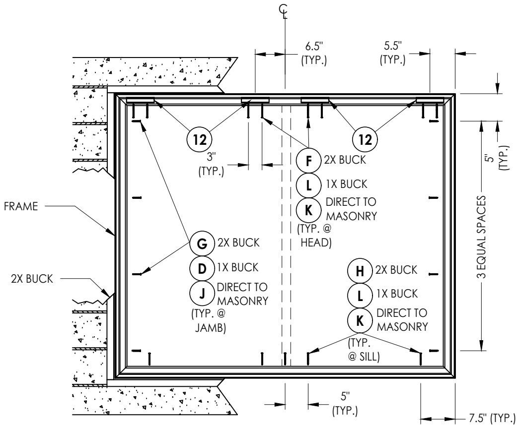
FRAME ANCHORING
