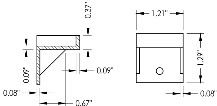
19 FLANKER STOP
