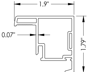
3 LOCK STILE
