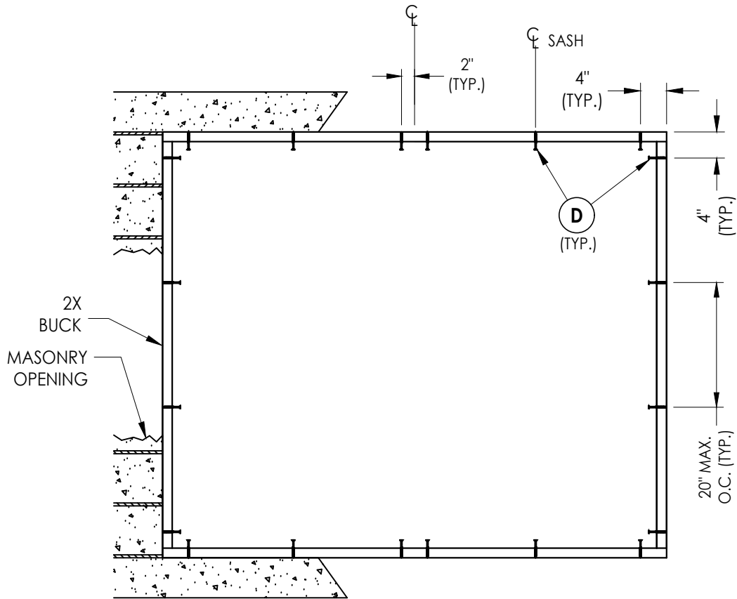
BUCK ANCHORING
